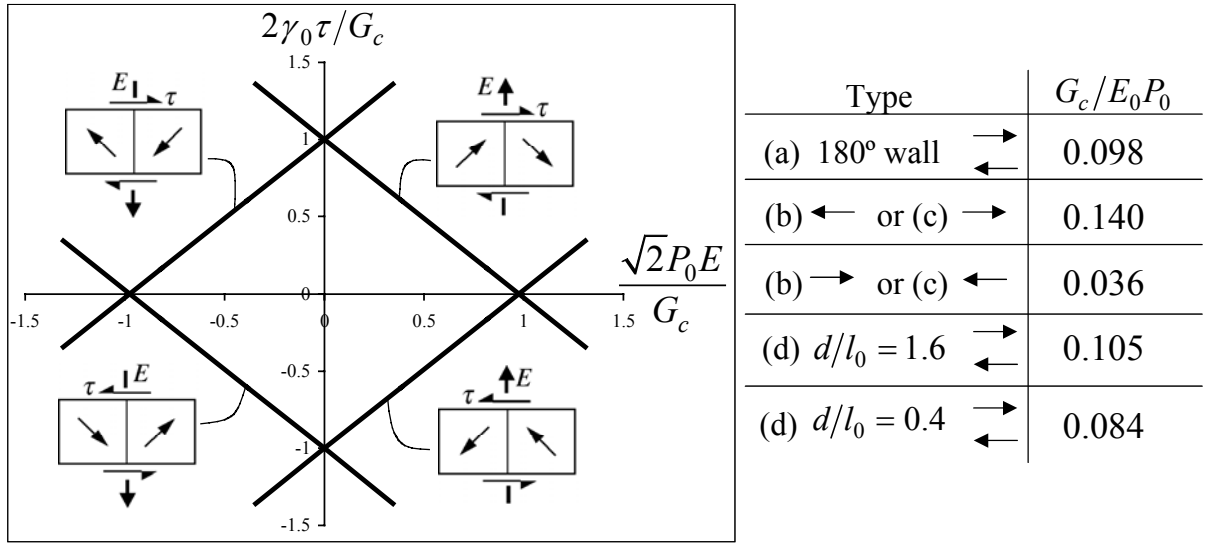
Figure 9. The “switching surface” for each of the three 90^\circ domain wall types and motion directions. The line charges have magnitude Q = 0.32P_0l_0 and are separated by h = 6.3l_0 . The linear relationships between the critical combinations of shear stress and the electric field have not been assumed but rather verified by the simulations. The table lists the critical energy density G_c required to break through the array for each of the domain wall/charge array interactions depicted in Figure 4.
