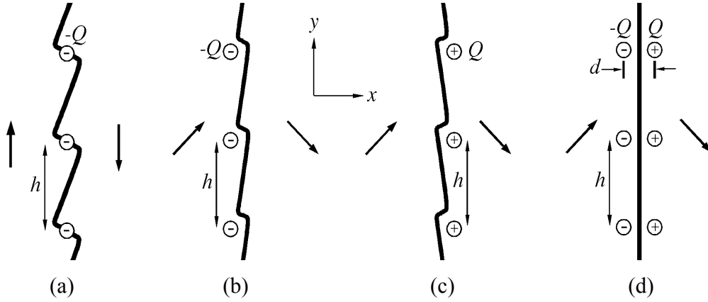
Figure 4. The configurations investigated for the interactions of domain walls with arrays point charge defects are illustrated above. (a) A 180^\circ wall with an array of negative point charges. The interaction of a 180^\circ wall with an array of positive point charges is mirror symmetric to the negative charge array. (b) A 90^\circ wall with an array of negative point charges. (c) A 90^\circ wall with an array of positive point charges. (d) A 90^\circ wall with an array of point charge dipoles. Results for the critical electric field and stress combinations for the wall to break through the array are presented in later figures.
