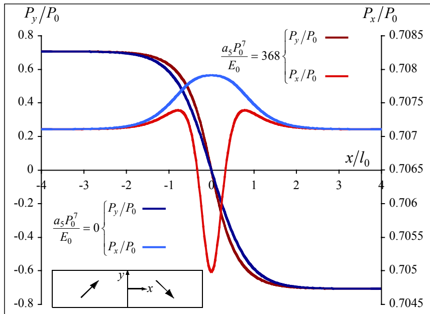
Figure 2a. The polarization distributions near a stationary 90^\circ domain wall for two different values of the parameter a_5 . The y -component of the polarization is given on the left ordinate axis and the x -component is given on the right ordinate axis. Note that the variations in P_x are relatively small, but result in large compensating levels of E_x (see Figure 2b). The arrows in the small inset figure nominally represent the polarization on either side of the domain wall located at x = 0 .
