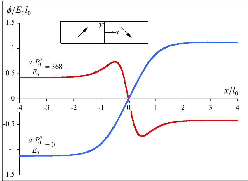
Figure 2c. The electric potential distributions near a stationary 90^\circ domain wall for two different values of the parameter a_5 . Note that there is a jump in the electric potential across the domain wall and the sign of the jump and shape of the distribution are sensitive to the material parameter a_5 . The arrows in the small inset figure nominally represent the polarization on either side of the domain wall located at x = 0 .
