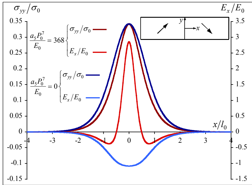
Figure 2b. The stress and electric field distributions near a stationary 90° domain wall for two different values of the parameter a_5 . The axial stress is given on the left ordinate axis and the x -component of the electric field is given on the right ordinate axis. The arrows in the small inset figure nominally represent the polarization on either side of the domain wall located at x = 0 .
