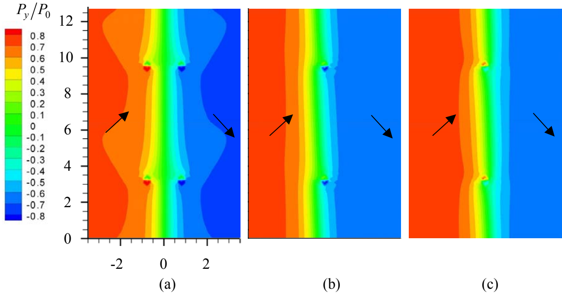
Figure 8. The P_y/P_0 polarization distribution near a 90^\circ domain wall interacting with an array of line charges, Q = 0.32P_0l_0 and h = 6.3l_0 . Red indicates polarization in the positive y -direction and blue in the negative y -direction. The x and y scales are normalized by l_0 . Periodic boundary conditions are enforced on the lines half of the distance between the charges. Electric field and shear stress are applied until the domain wall is able to break through the charge array. Figures a-c depict the equilibrium domain wall configuration for applied field levels of (a) d = 1.6l_0 , E = 0 and \tau = 0 for the configuration from Figure 4a, (b) E = 0 and \tau = 0 for the configuration from Figure 4c, and (c) E = 0 and \tau = 0.159\sigma_0 for the configuration from Figure 4c. The load level in (c) is very close to the breaking strength for this particular charge dipole array.
