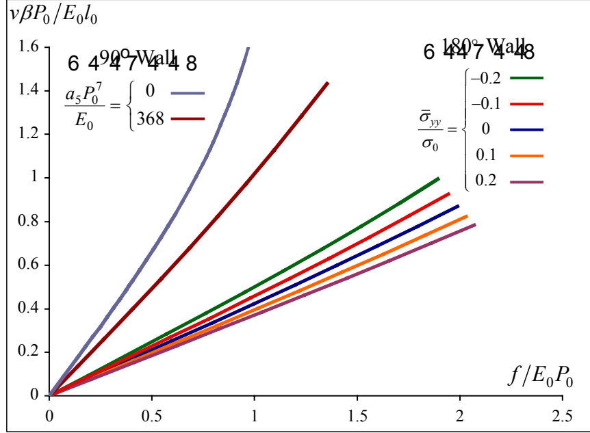
Figure 3. Domain wall velocity versus the Eshelby driving traction for a 180° domain wall under different levels of applied stress, and for 90° domain walls in materials with different a_5 coefficients. For each level of the average applied stress \bar{\sigma}_{yy} the driving force for the 180° wall is controlled solely by E_y , however each of the curves for the 90° walls contain data points from multiple combinations of applied electric field E_y and shear stress \sigma_{xy} .
