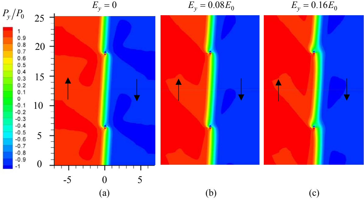
Figure 5. The P_y/P_0 polarization distribution near a 180^\circ domain wall interacting with an array of line charges. The lines are negatively charged at a level of Q = 1.26P_0l_0 , separated by a distance h = 12.6l_0 , and can be seen as the small red and blue circles. Red indicates polarization in the positive y -direction and blue in the negative y -direction. The x and y scales are normalized by l_0 . Periodic boundary conditions are enforced on the lines half of the distance between the charges. Electric field is applied in the y -direction until the domain wall is able to break through the charge array. Figures a-c depict the equilibrium domain wall configuration for applied field levels of (a) E_y = 0 , (b) E_y = 0.08E_0 and (c) E_y = 0.16E_0 . The field level in (c) is very close to the breaking strength for this particular charge array.
