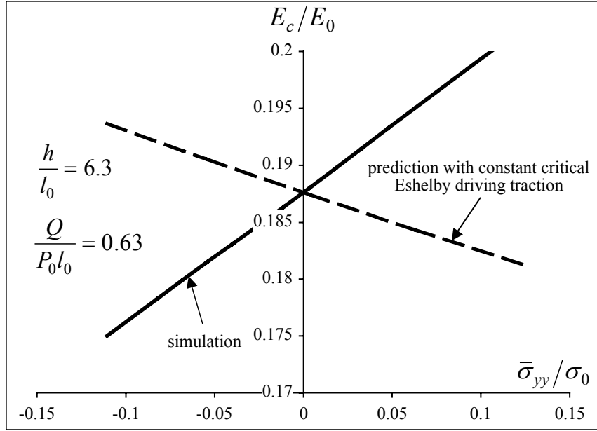
Figure 7. The effects of an applied axial stress along the nominal domain wall direction on the critical electric field required for a 180^\circ domain wall to break through the charge array.
