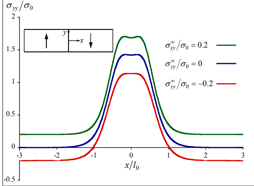
Figure 1b. The axial stress distribution near a stationary 180^\circ domain wall for levels of far field applied stress of \sigma_{yy}^\infty/\sigma_0 = -0.2, 0 , and 0.2 . The arrows in the small inset figure nominally represent the polarization on either side of the domain wall located at x = 0 .
