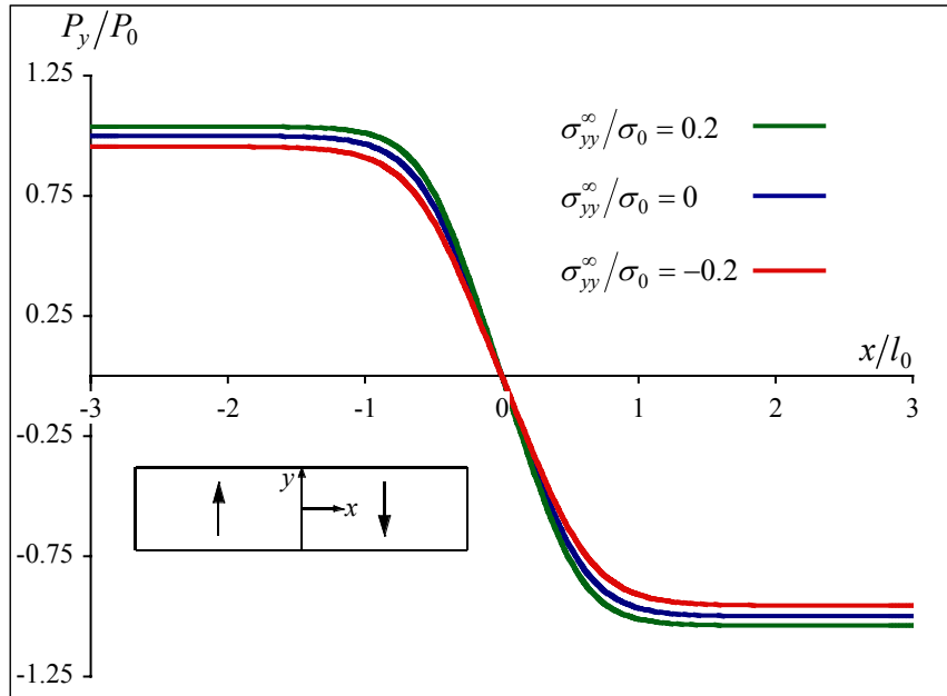
Figure 1a. The polarization distribution near a stationary 180^\circ domain wall for levels of far field applied stress of \sigma_{yy}^\infty/\sigma_0 = -0.2, 0 , and 0.2 . Note that the thickness of the domain wall is approximately 2l_0 , where l_0 = \sqrt{a_0 P_0/E_0} . The arrows in the small inset figure nominally represent the polarization on either side of the domain wall located at x = 0 .
