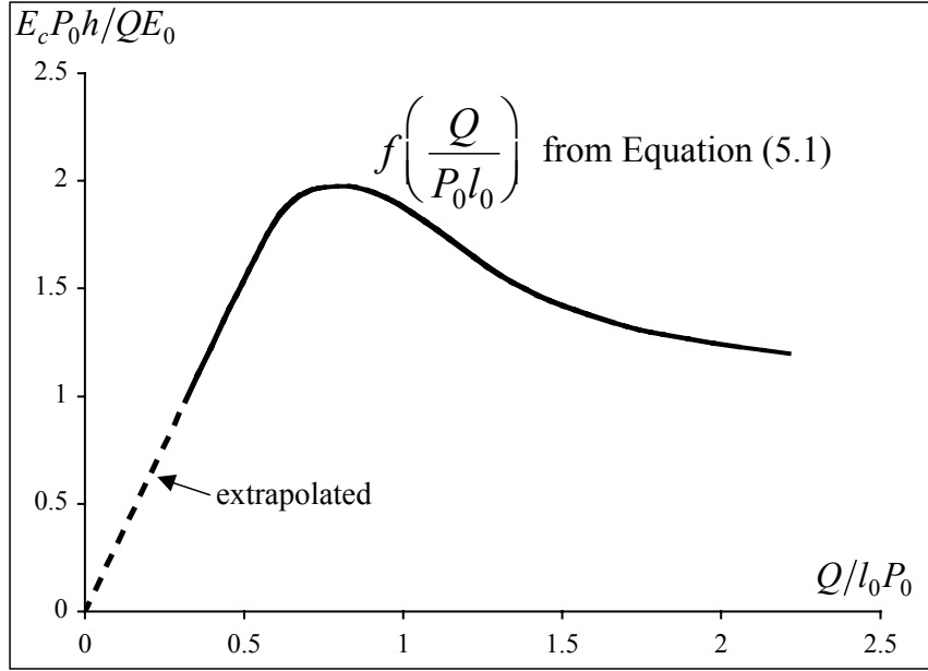
Figure 6. The critical electric field E_c required for a 180^\circ domain wall to break through an array of charge defects of the configuration illustrated in Figure 4a has a 1/h dependence as given in Equation (5.1). The dimensionless function f is of order unity and is plotted here.
